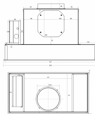
Metz Micro 534 - internal motor
